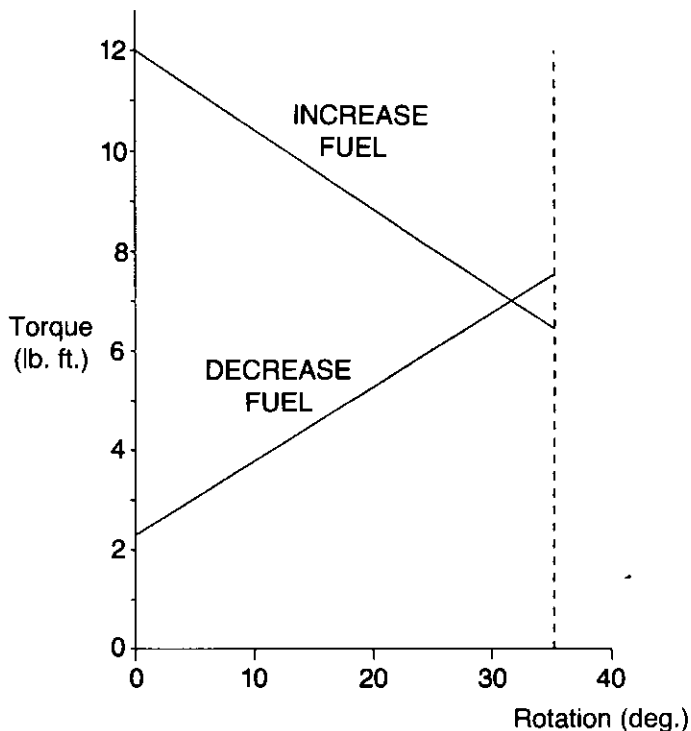
Figure 1 Actuator Torque
